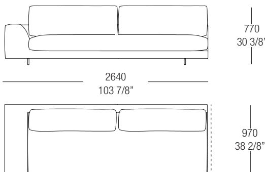
AG23TLUD/S cuscino seduta intero. full sitting cushion.
