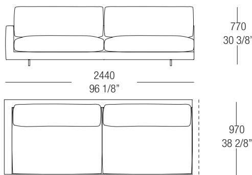
AG23TSD/S cuscino seduta diviso. split sitting cushion.
