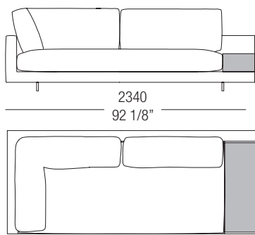
AG19AEUD/S cuscino seduta intero. full sitting cushion.
