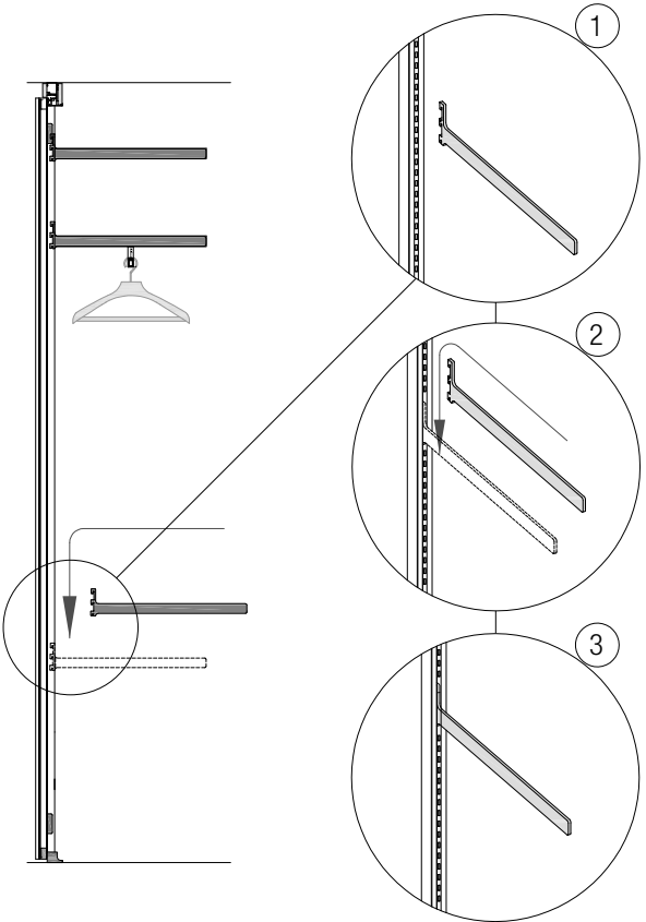
Details bracket hooks (1,2 e 3)
