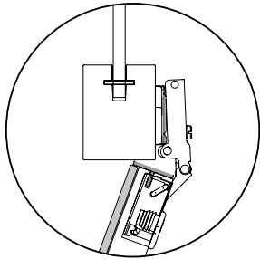
94° STANDARD HINGE fixed on the upright
