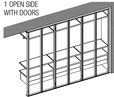
UNIT WITHOUT DOORS IN CENTRE ROOM
